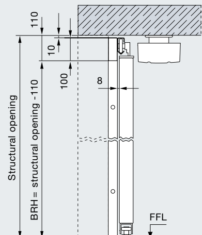
Vertical section
