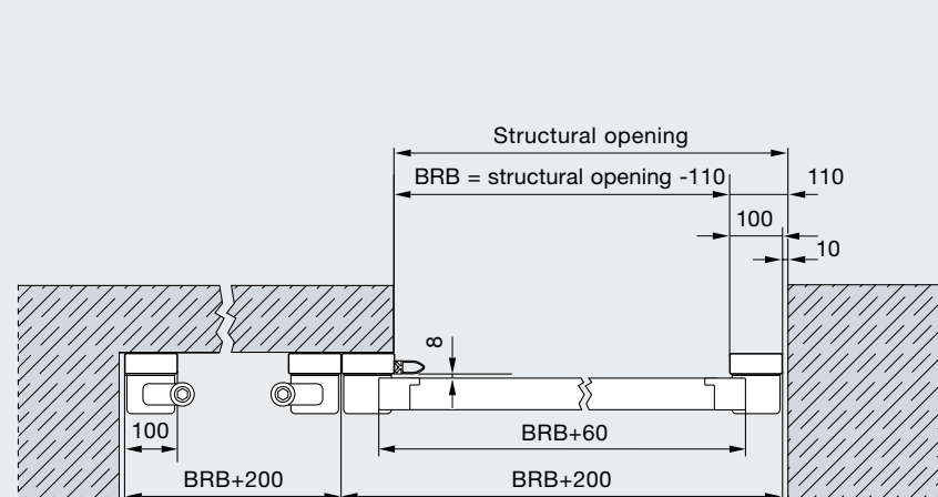
Horizontal section
