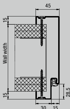
Profile 21120 Screw-fixing
