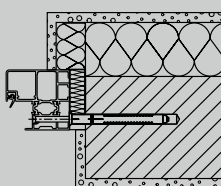
Fitting versions
