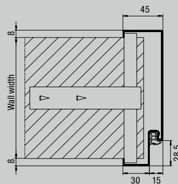
Profile 21101
