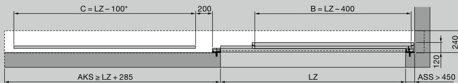
Wall fitting (floor rail view)
