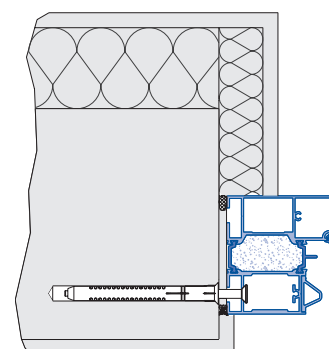
Aluminium frame Countersunk fitting shown (drill holes on site)
